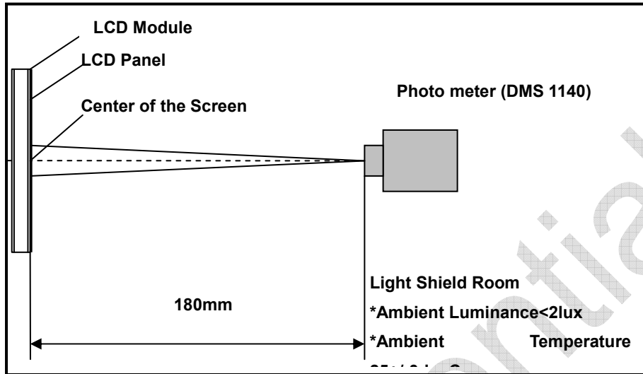
Figure 3 Measurement Setup
