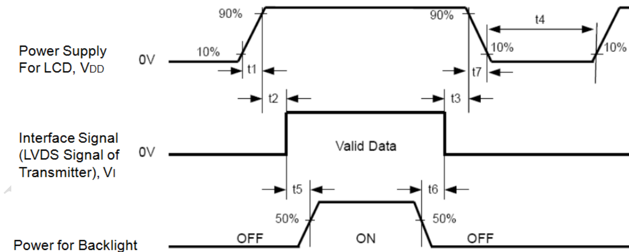
Figure 13 Power Sequence
