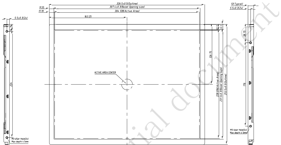
Figure 14 Reference Outline Drawing (Front Side)
