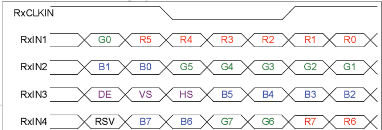
Figure 10 Data Mapping
