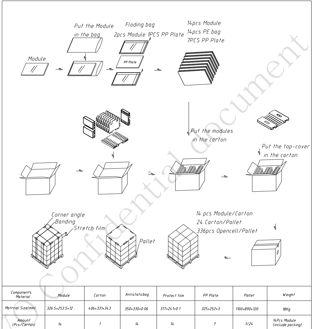
Figure 17 Packing Method
