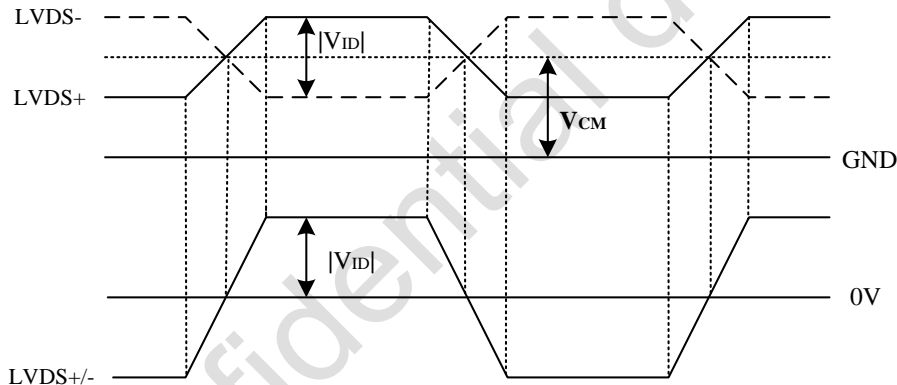
Figure 8 Voltage Definitions
