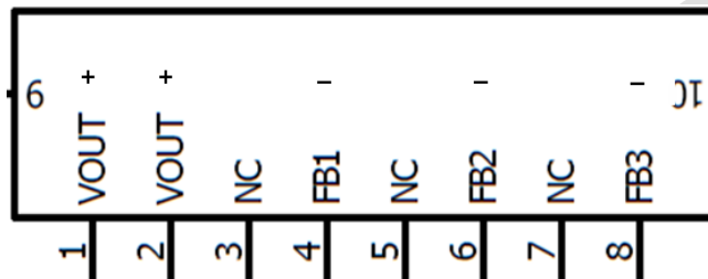
Figure 7 LED Connector
