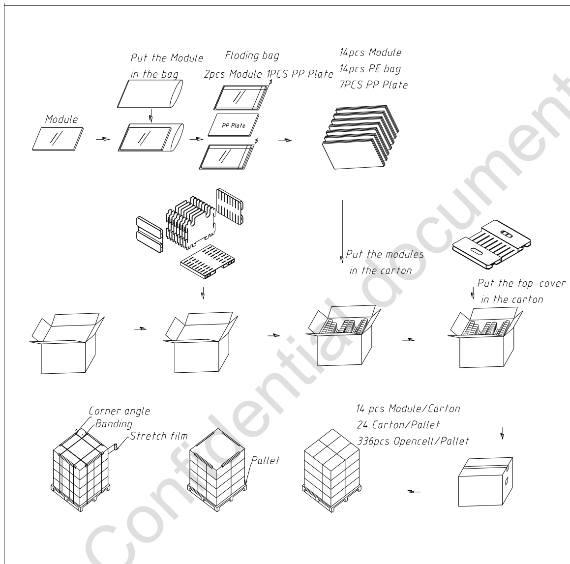
Figure 16 Packing Method
