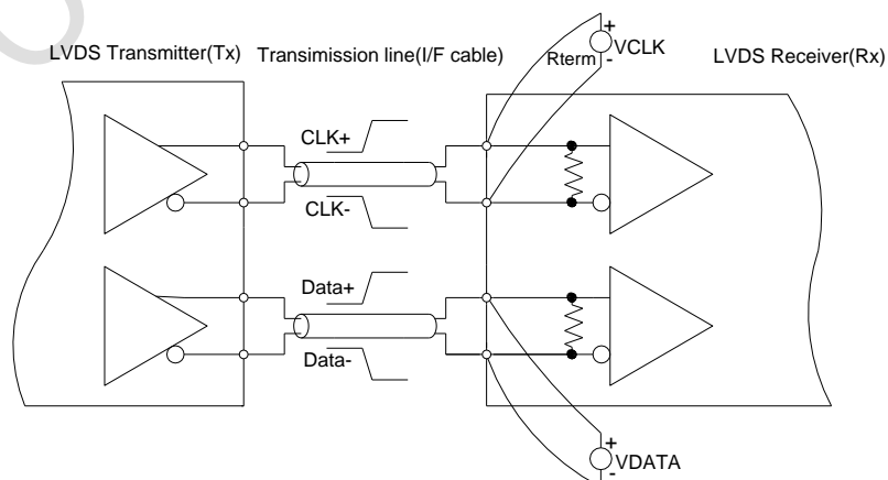
Figure 9 Measurement System
