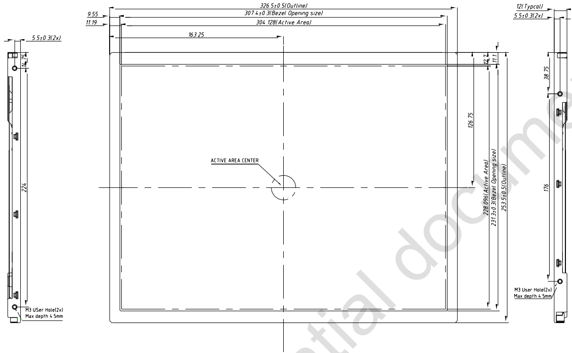
Figure 15 Reference Outline Drawing (Back Side)
