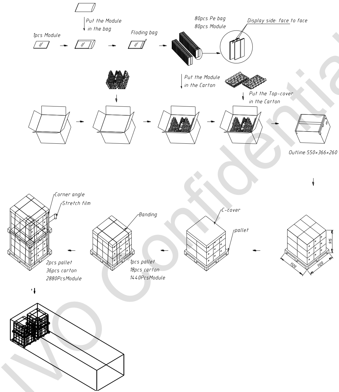
Figure 14 Packing Method
