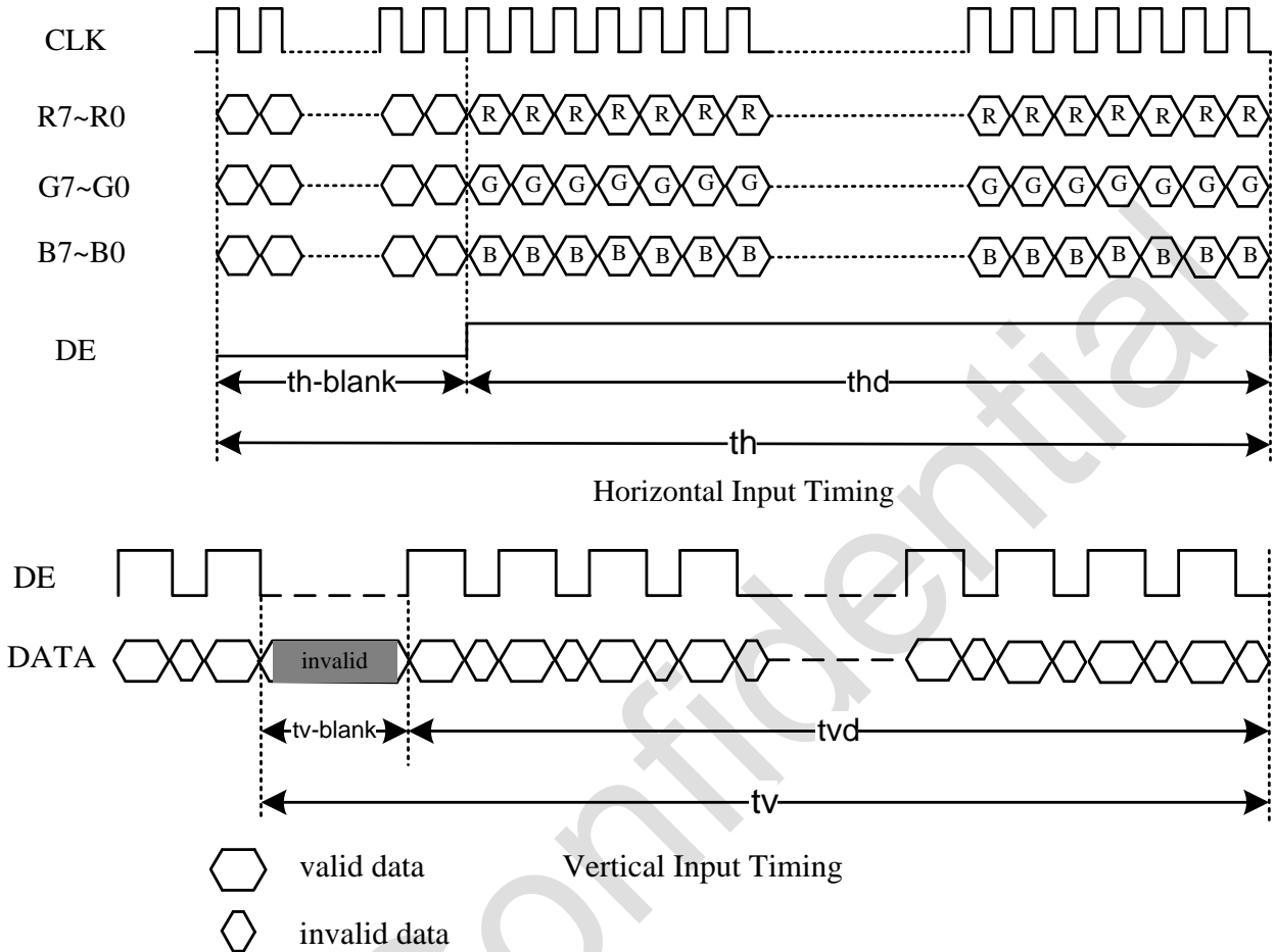
Figure 7 Timing Characteristics
