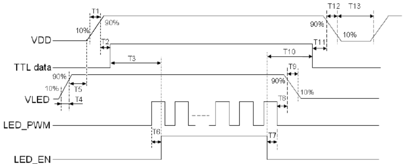
Figure 10 Power Sequence
