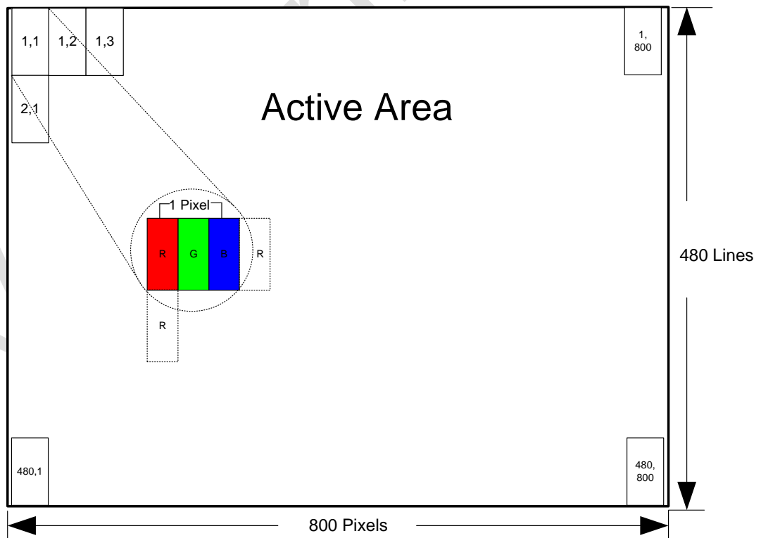
Figure2 Pixel Mapping
