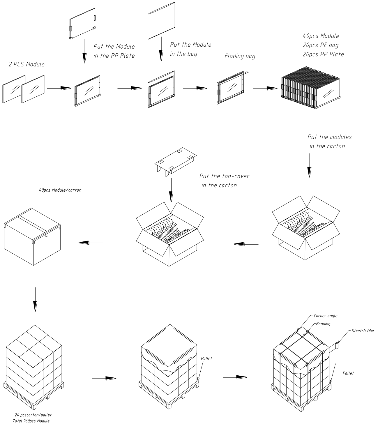
Figure 16 Packing Method
