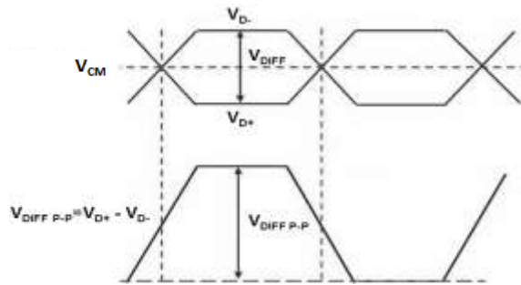
Figure 10 Display Port AUX_CH Signal
