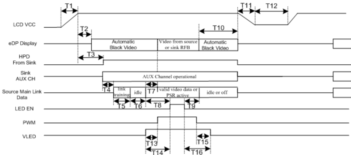
Figure 13 Power Sequence
