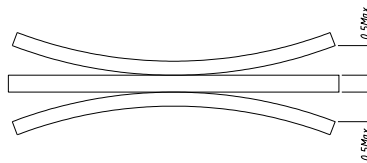
LCM Warpage Schematic
