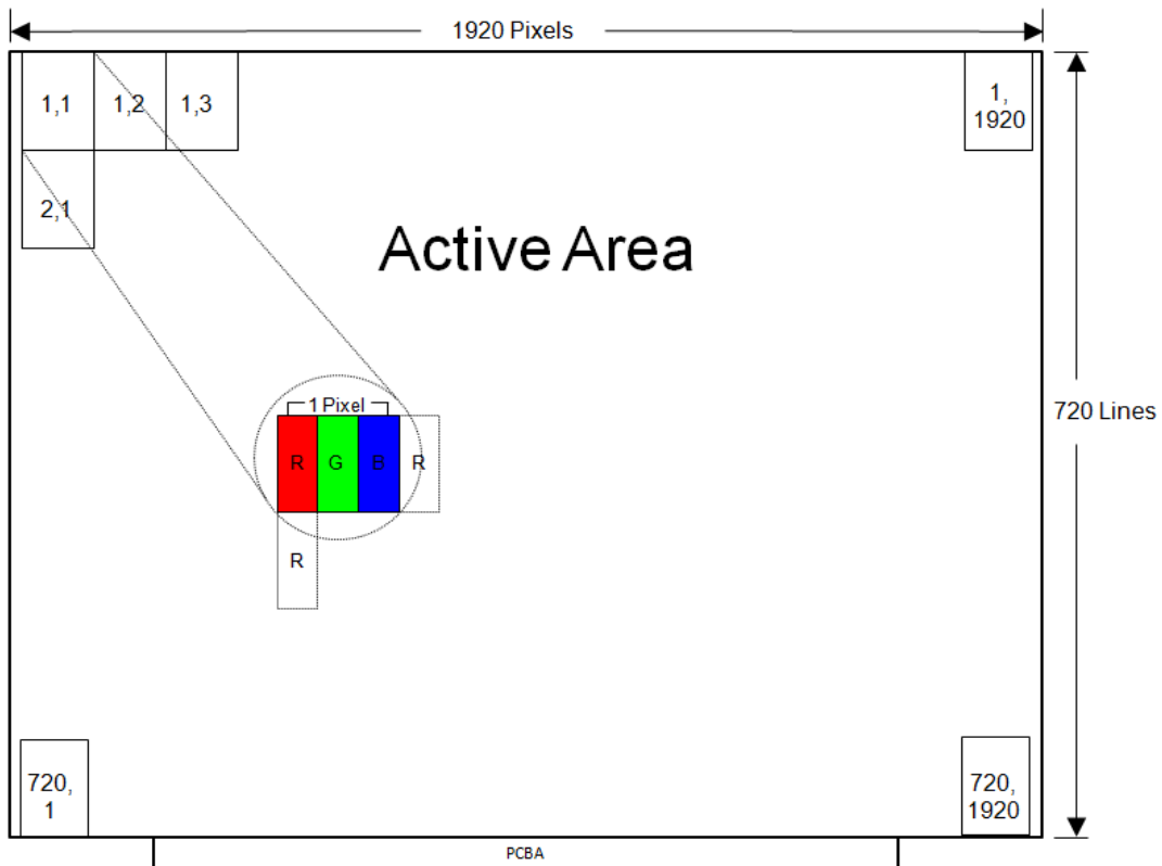
Figure2 Pixel Mapping
