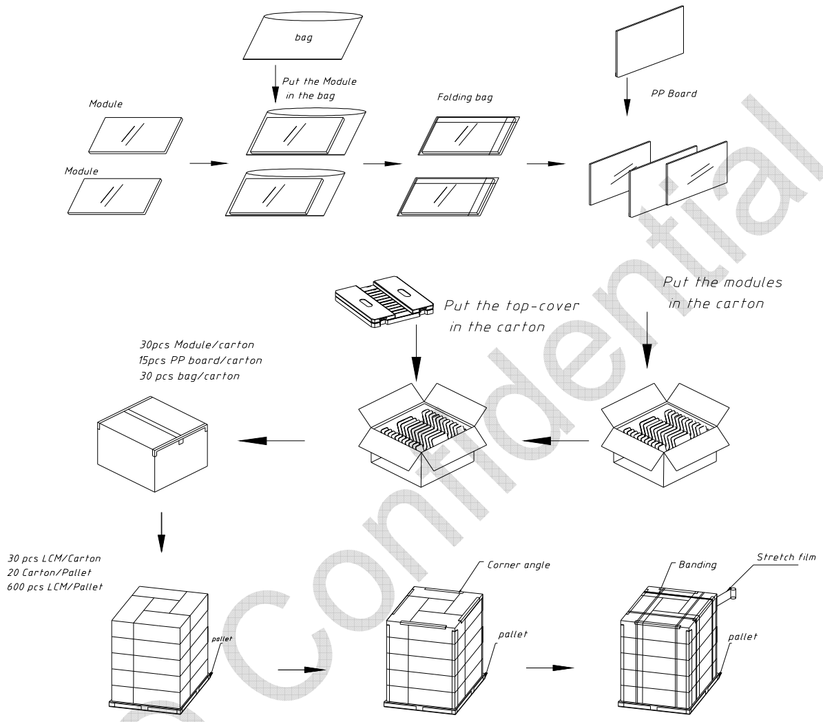
Figure 18 Packing Method
