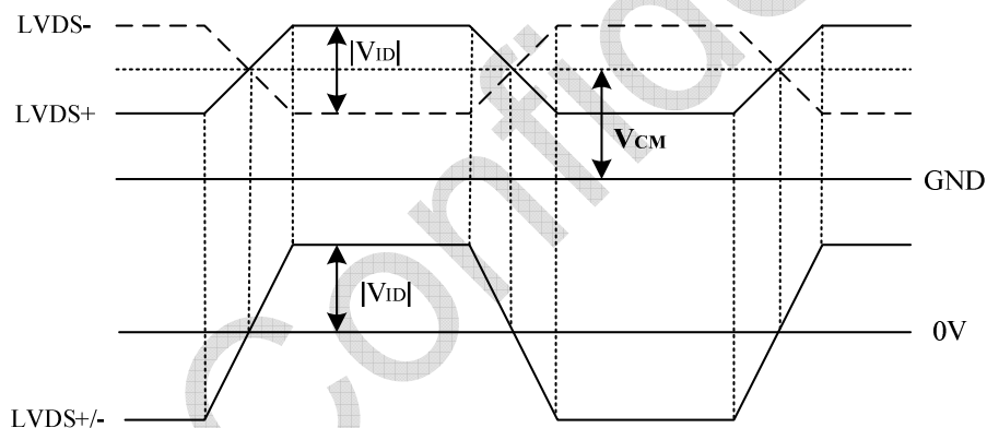
Figure 8 Voltage Definitions
