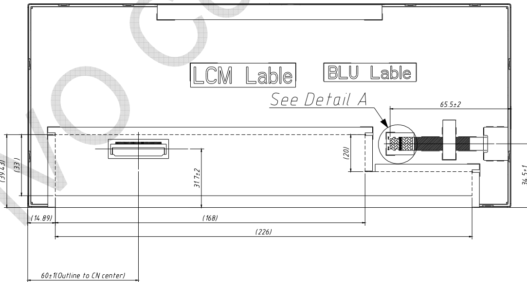
Figure 15 Reference Outline Drawing (Back Side)
