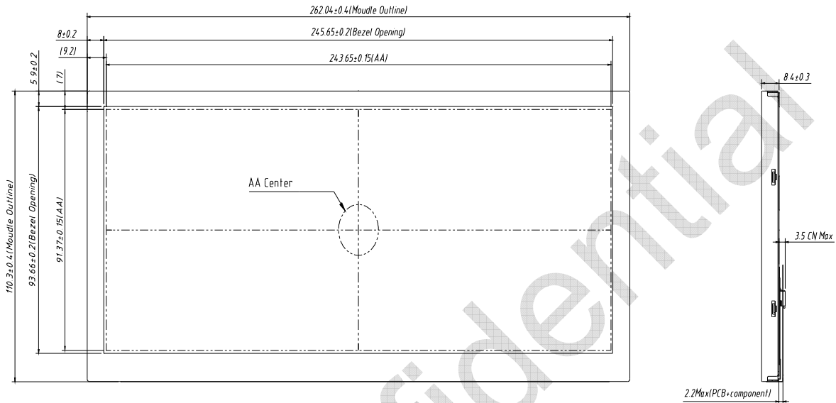
Figure 14 Reference Outline Drawing (Front Side)
